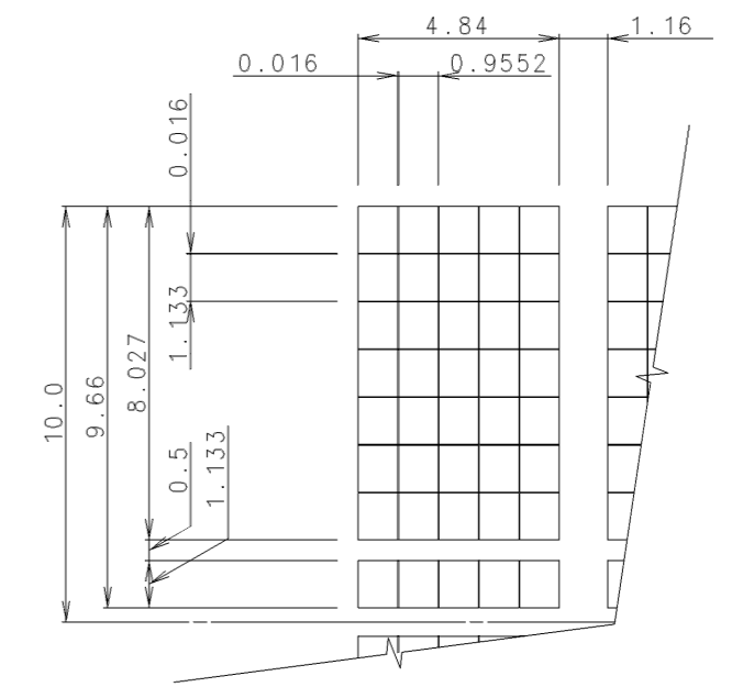
DOT DETAIL (SCALE 5:1)
