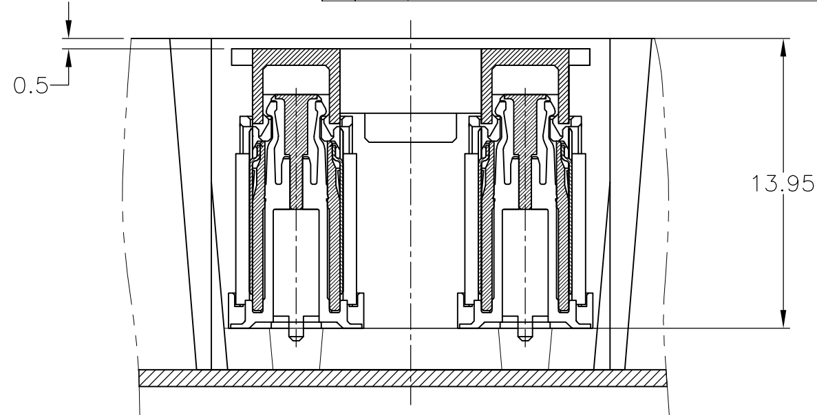
E-E (SCALE 4:1)
