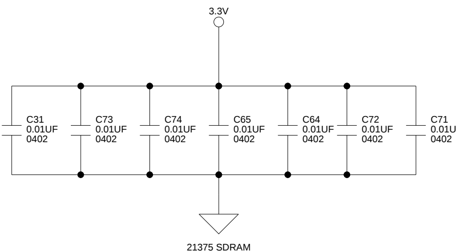
21375 SDRAM
