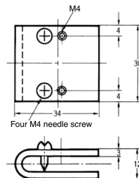
F03-08 End Cap (Neoprene Rubber)
