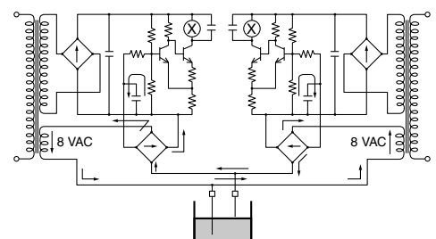
Fig. 1 Internal Closed Circuit
