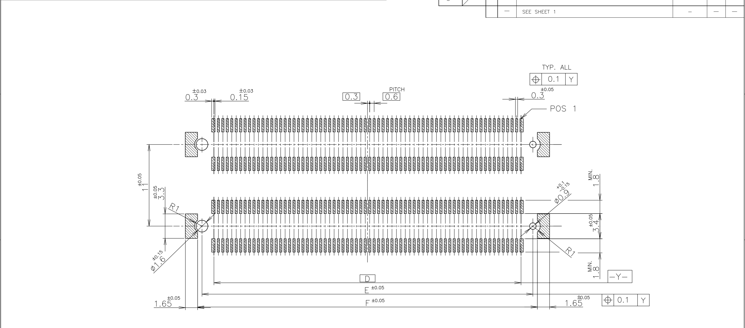
REFERENCE P.C.BOARD LAYOUT
