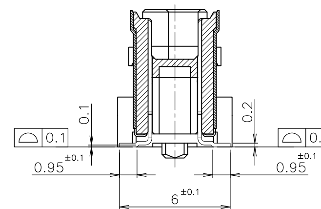
A-A (SIGNAL POSITION) (SCALE 5:1)
