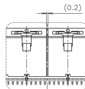
DETAIL C 180P~240P ONLY
