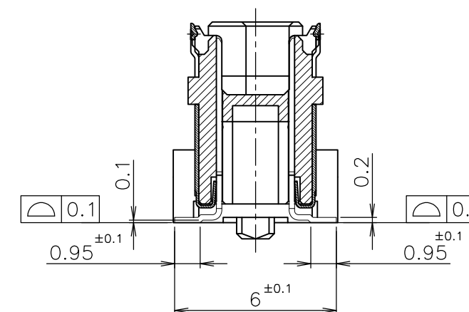
B-B (GROUND POSITION) (SCALE 5:1)
