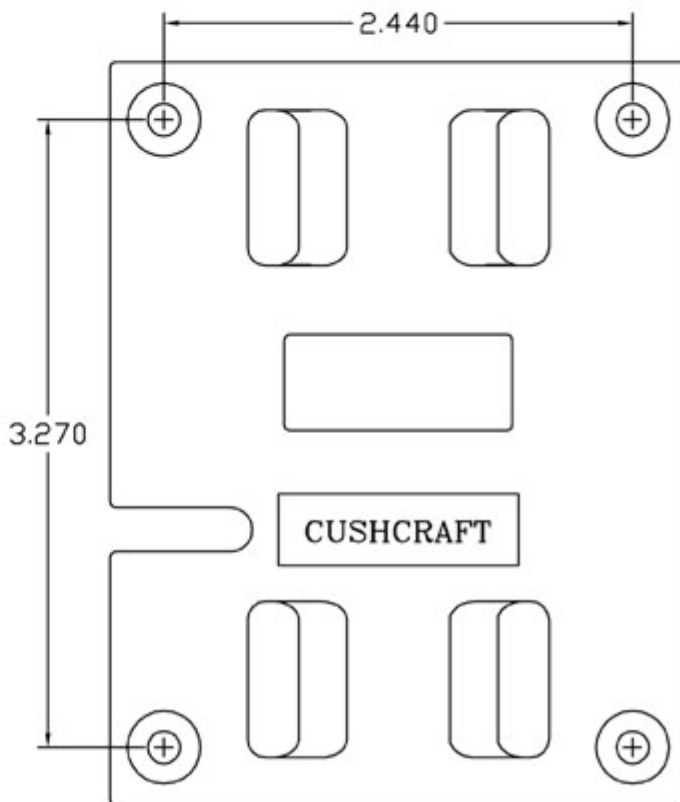
DRILL TEMPLATE
