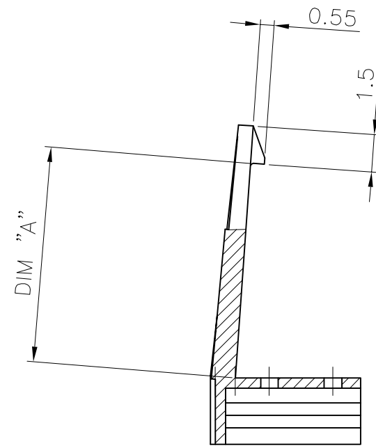
SECTION Z-Z
