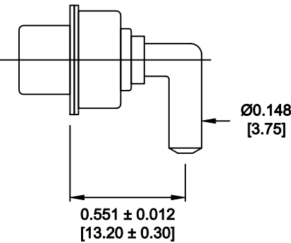
40 AMP POWER CONTACT
