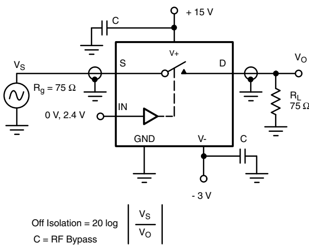
Figure 4. Off Isolation
