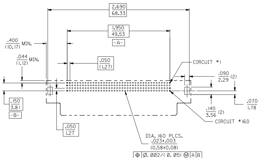
RECOMMENDED PC BOARD LAYOUT COMPONENT SIDE
