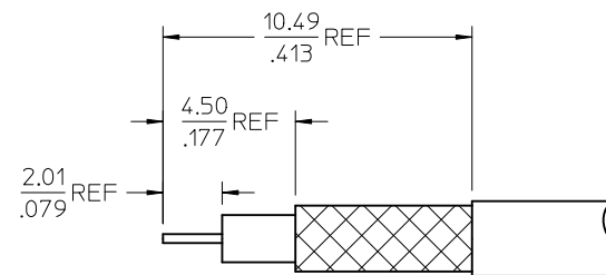
RECOMMENDED CABLE STRIP
