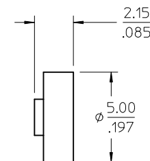
INSULATOR
