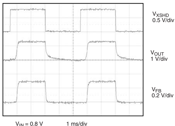
Figure 2. PWM Dimming Control 200 Hz 50 % Duty Cycle PWM Signal on XSHD Pin
