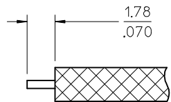
RG405 CABLE PREP
