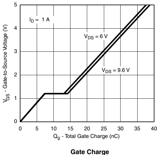
Gate Charge
