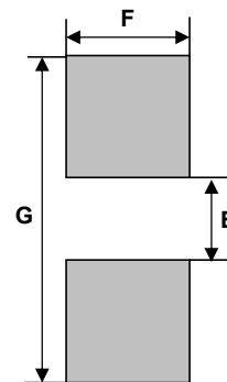
Land Pattern
