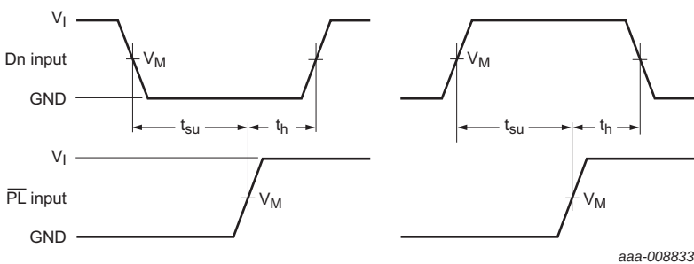
Measurement points are given in Table 8. Fig 11. Set-up and hold times from the data inputs (Dn) to the parallel load input ( \overline{PL} )
