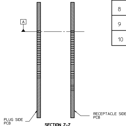
SECTION Z-Z
