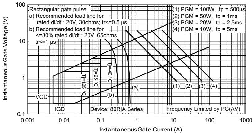
Fig. 9 - Gate Characteristics
