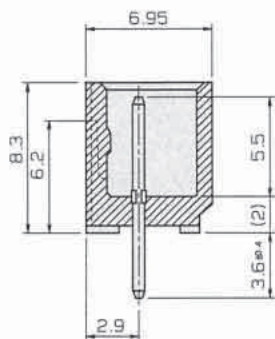
SECT. G-G
