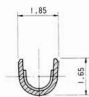
SECT. b~b
