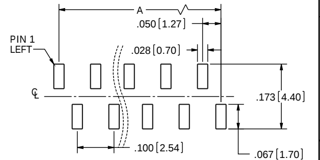
RECOMMENDED PCB LAYOUT LPPB_1NFS-RC
