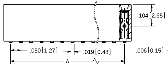
LPPB_1NFS-RC (OPPOSITE BEND, APPLICABLE ON EVEN PIN COUNTS)
