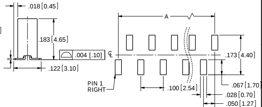
RECOMMENDED PCB LAYOUT LPPB_1NFS-RC
