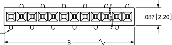
LPPB_1NFS-RC (OPPOSITE BEND, APPLICABLE ON EVEN PIN COUNTS)
