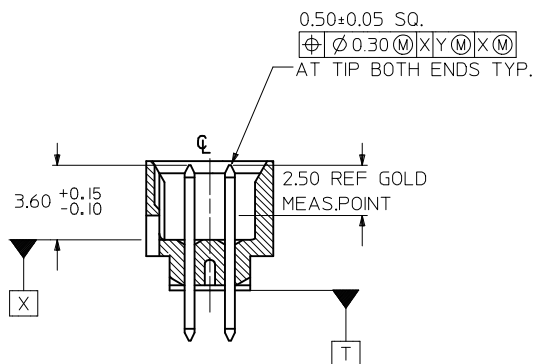
SECTION G-G
