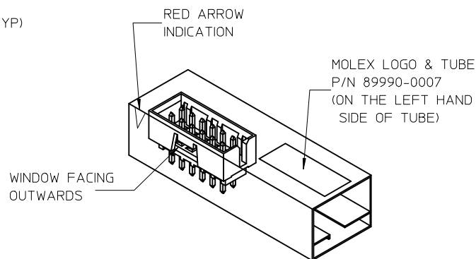
ORIENTATION OF PART IN TUBE.
