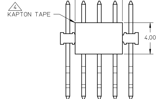
PART WITH KAPTON TAPE 10CKT SHOWN FOR ILLUSTRATION ONLY
