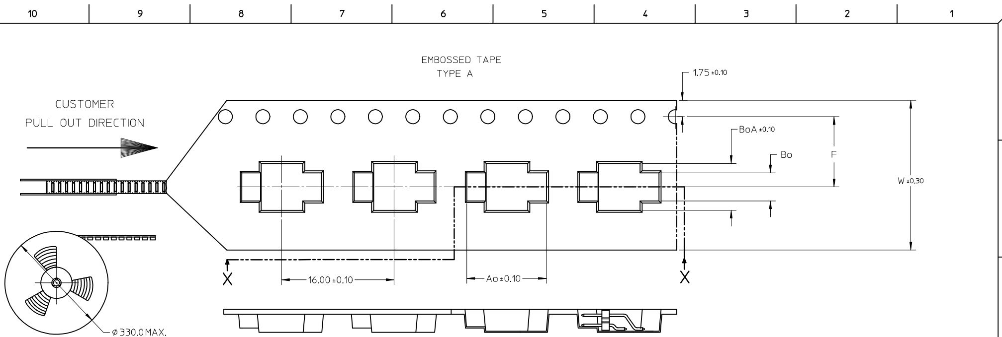
SECTION X-X PART IN T&R FOR ILLUSTRATION ONLY
