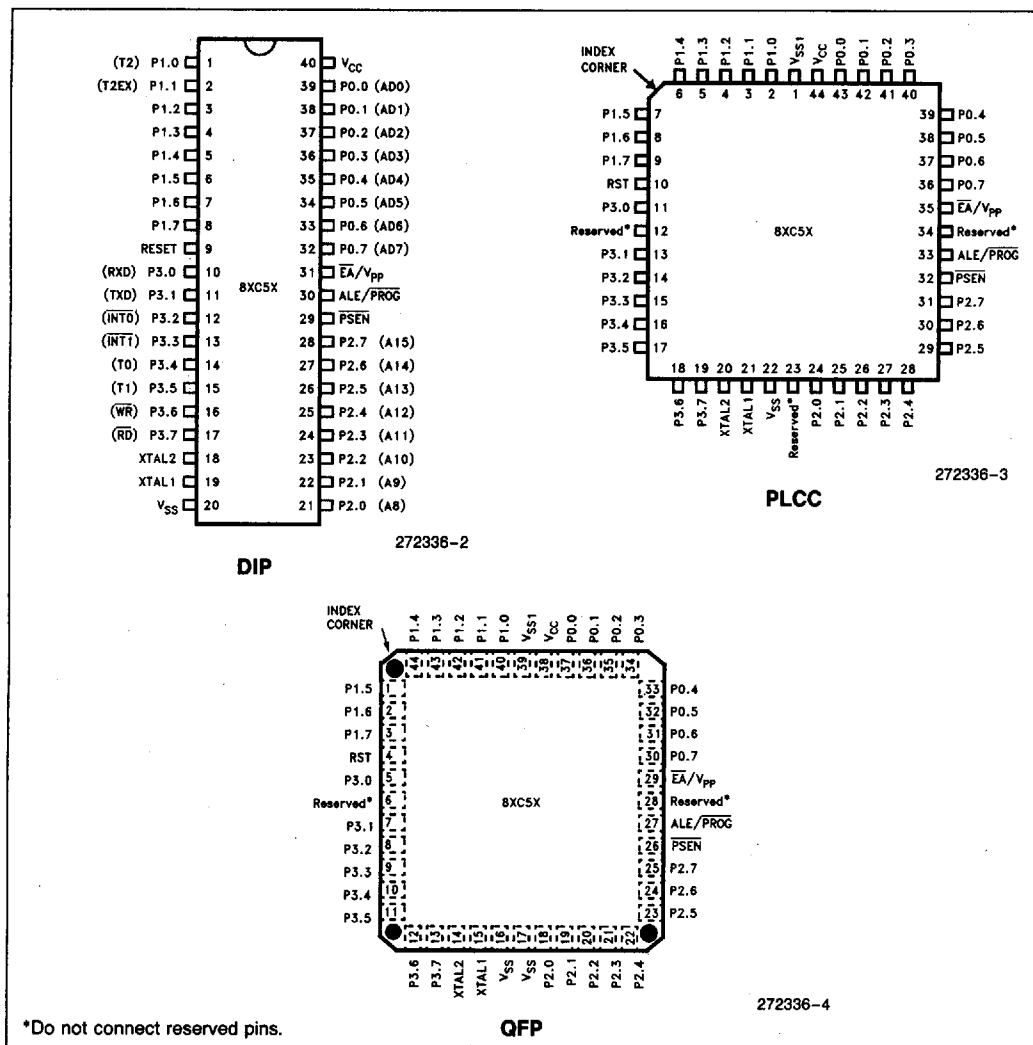
Figure 2. Pin Connections
