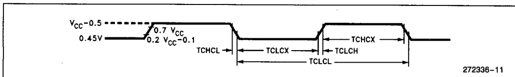
Figure 9. Clock Signal Waveform for I_{CC} Tests in Active and Idle Modes. TOLCH = TCHCL = 5 ns
