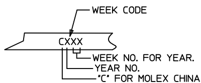
DETAIL C
