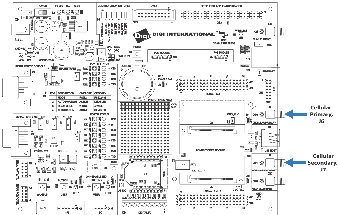
ConnectCore 9P 9215 Development Board
