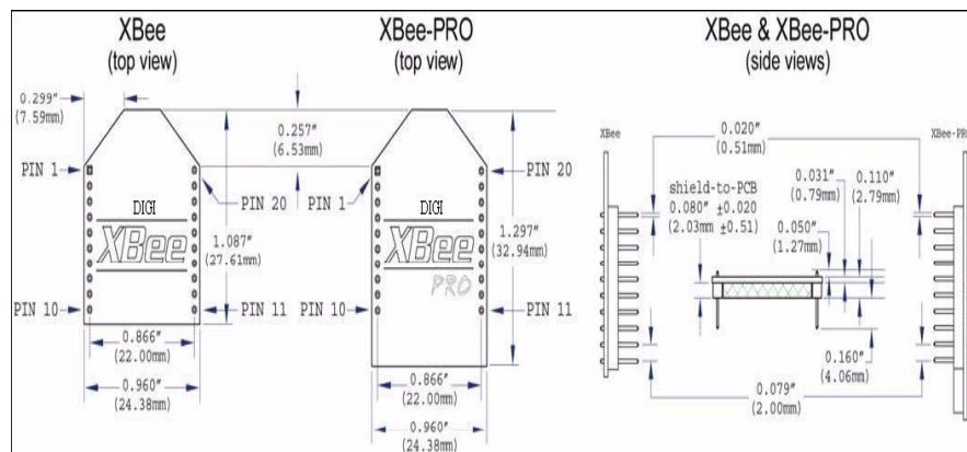
Figure 1-04. Mechanical Drawings
