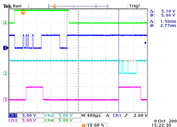
Figure 2-012. Binary Command Write then Read
