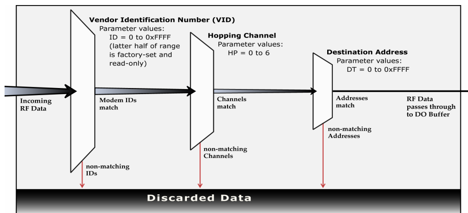
Figure 2-07. Addressing Layers contained in the Header
