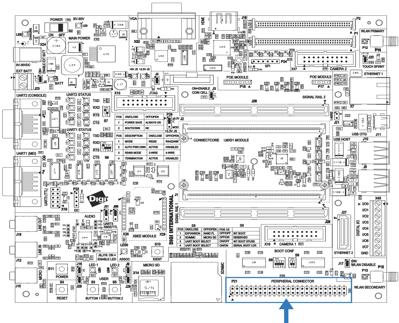
Peripheral Application Header, P21
