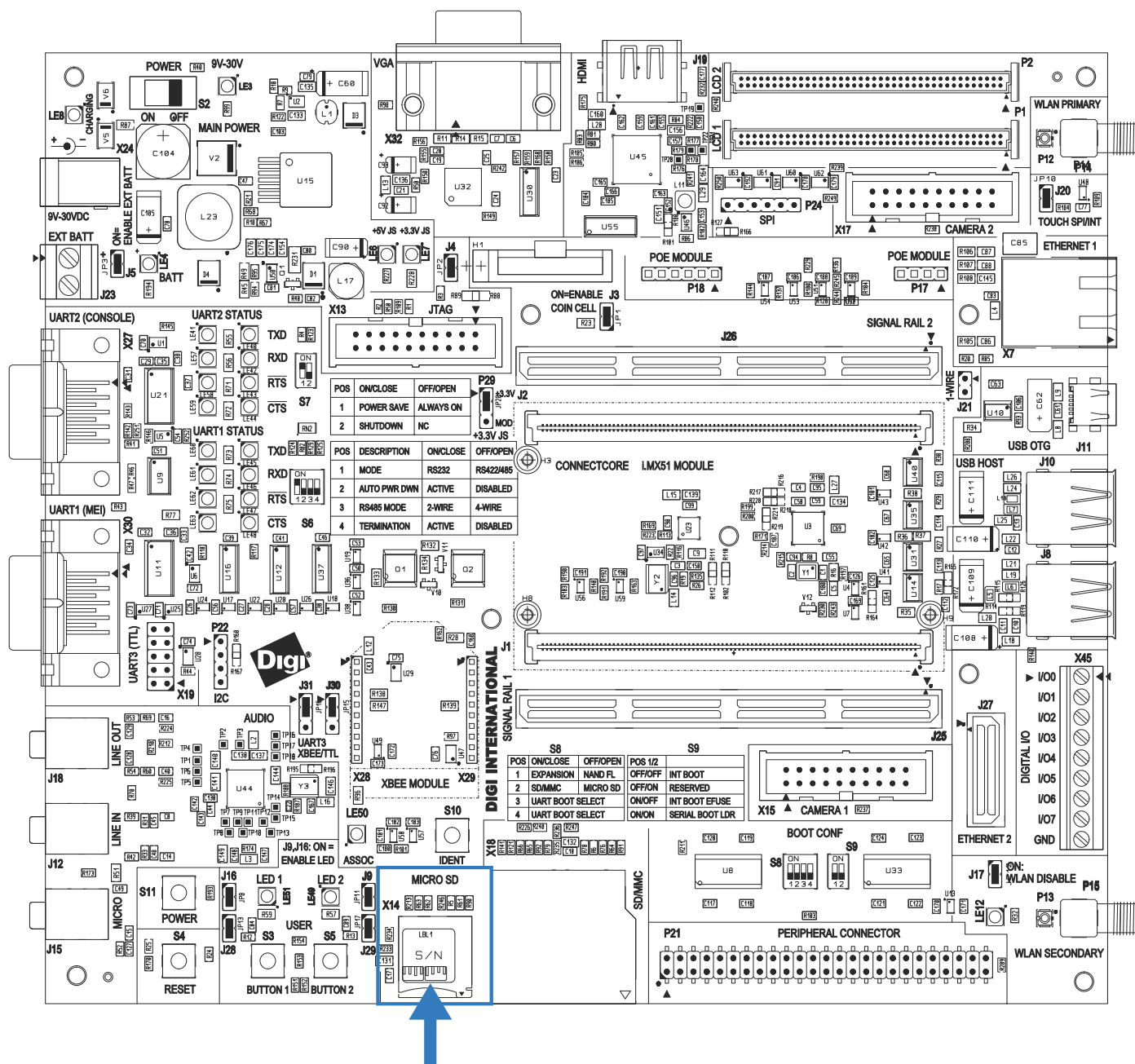
MicroSD Connector, X14
