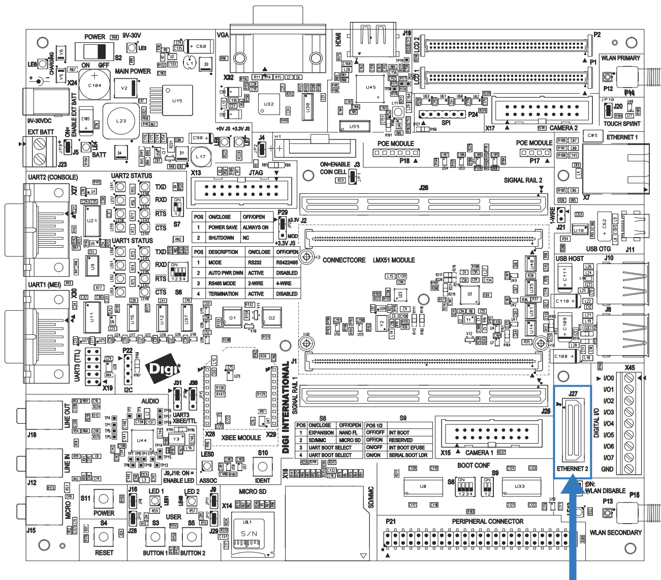
Ethernet 2 Connector, J27
