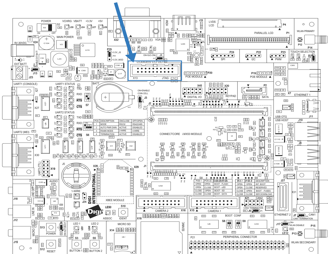
JTAG Connector, X13
