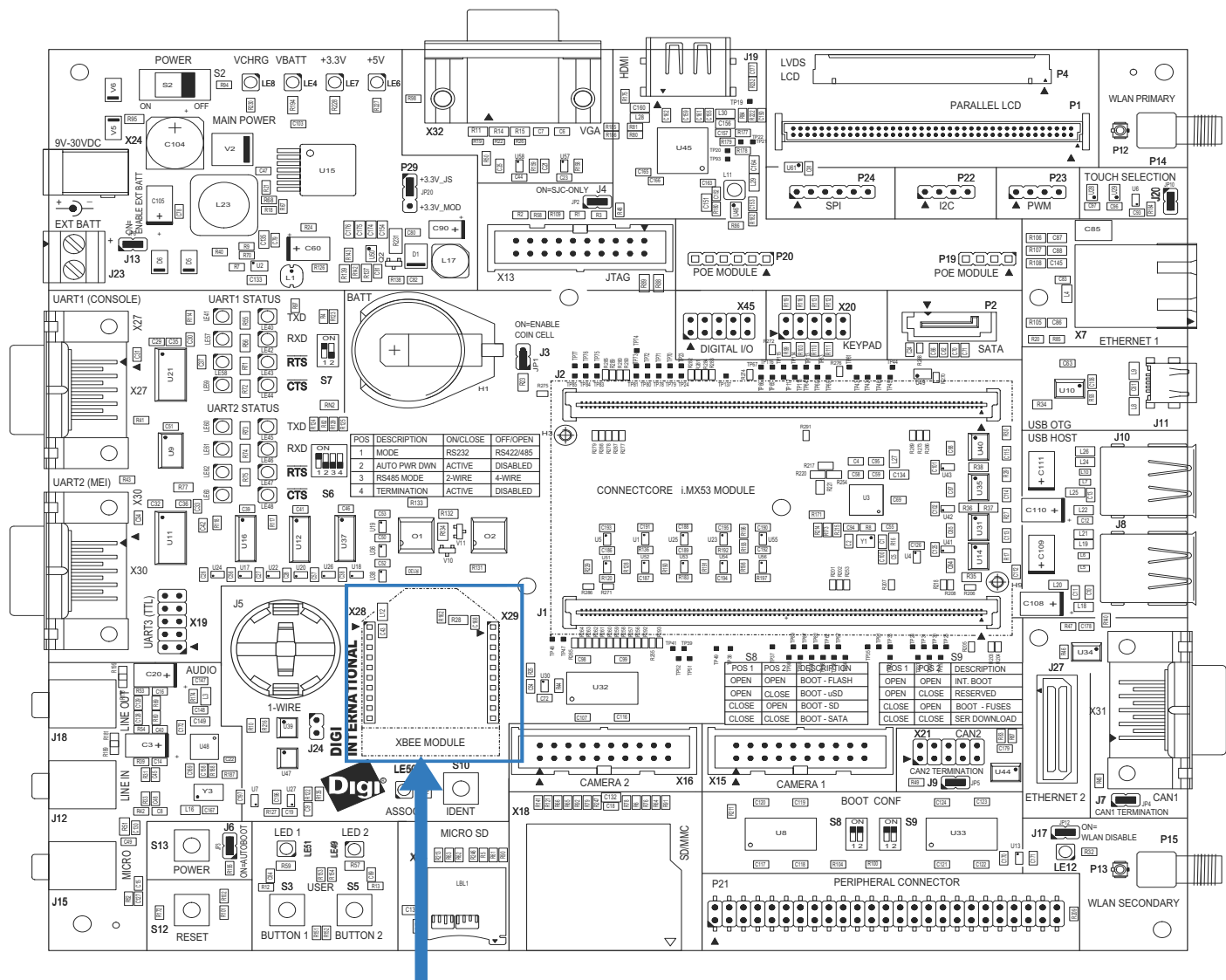
Digi XBee Connectors, X28 & X29
