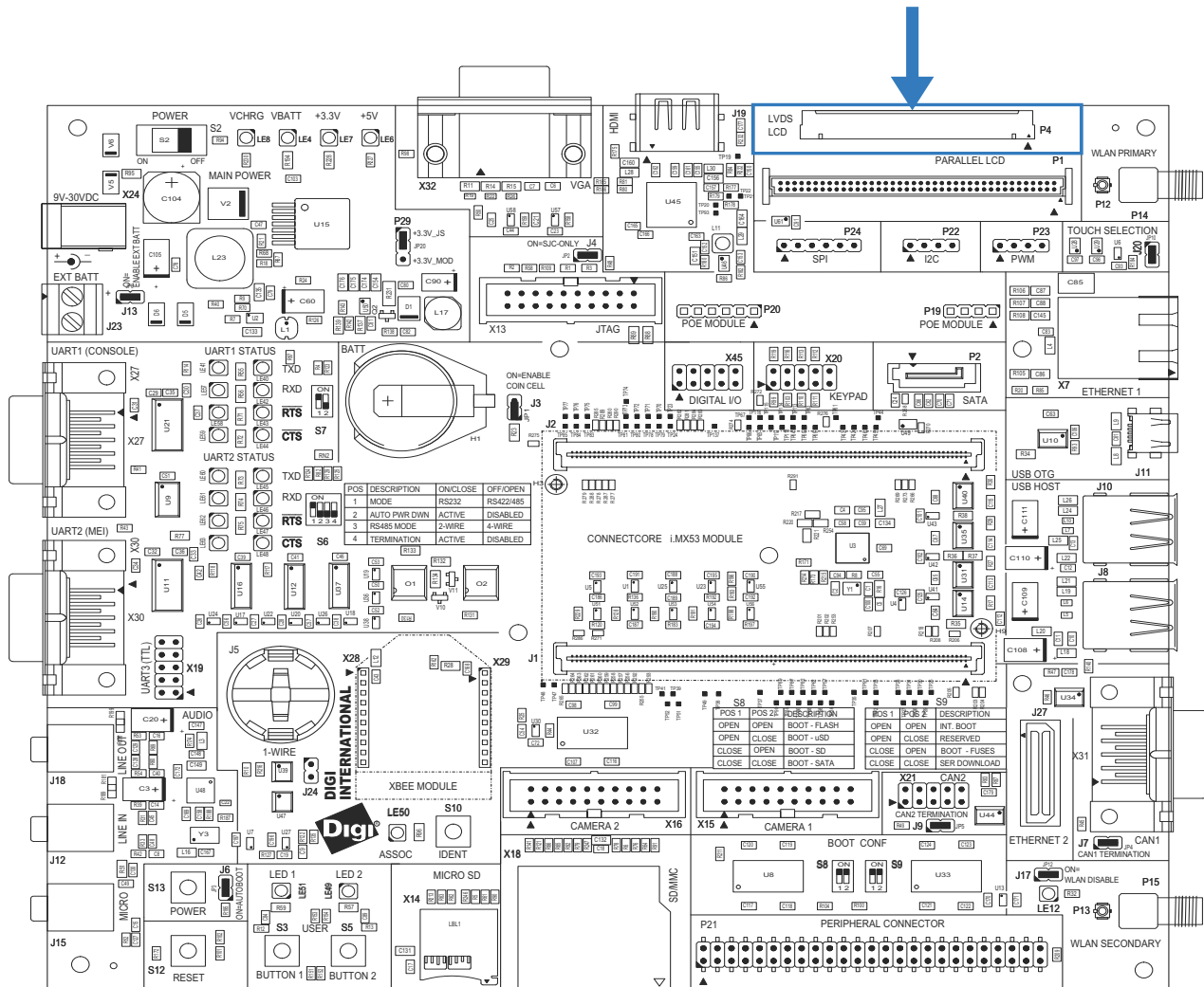
LVDS LCD Connector, P4
