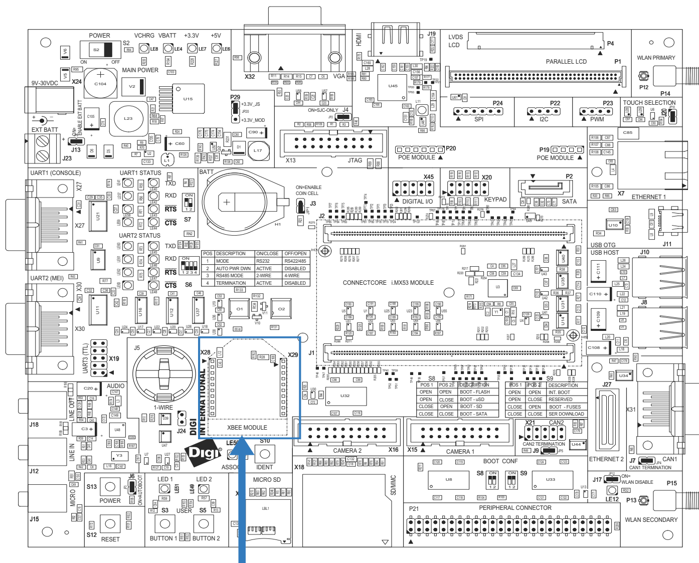
Digi XBee Connectors, X28 & X29
