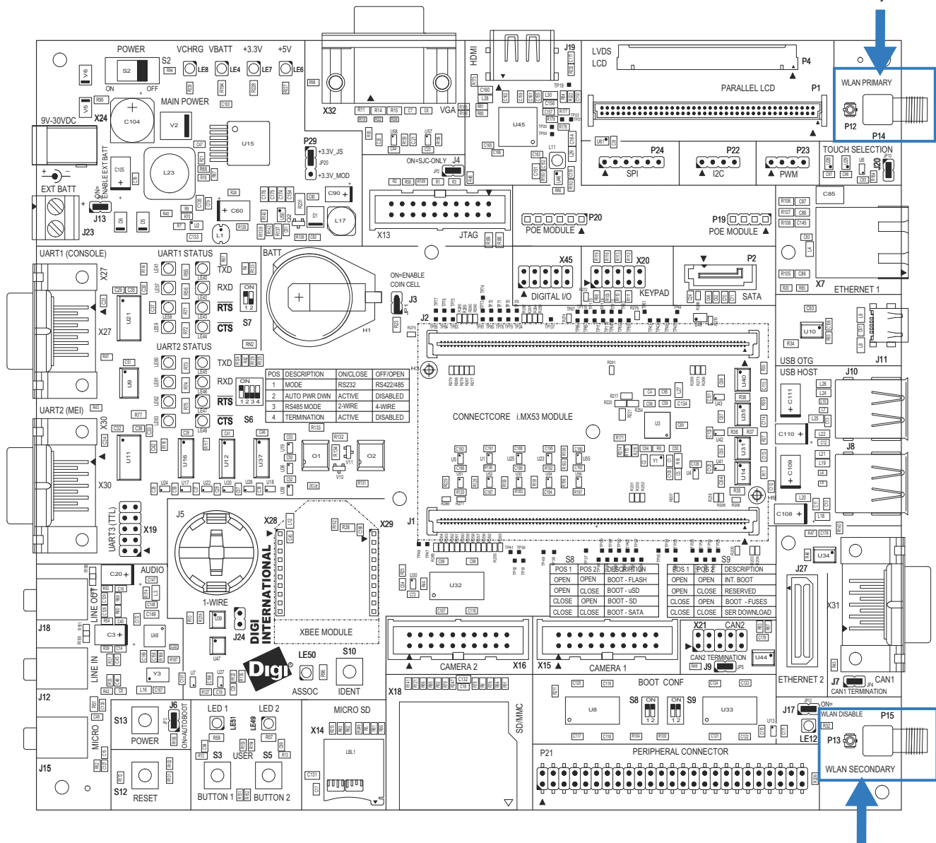
Secondary Antenna Connectors, P13 & P15
