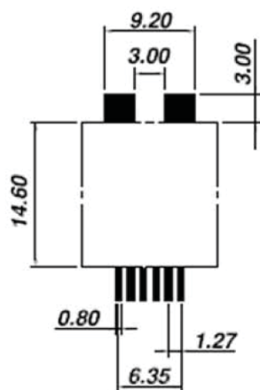
PBC Layout (Top View)
