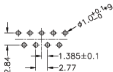
9 Pin Female Connector PCB Pin Layout
