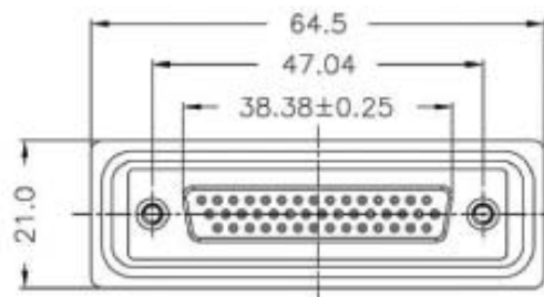
44 Pin Female Connector PCB Pin Layout
