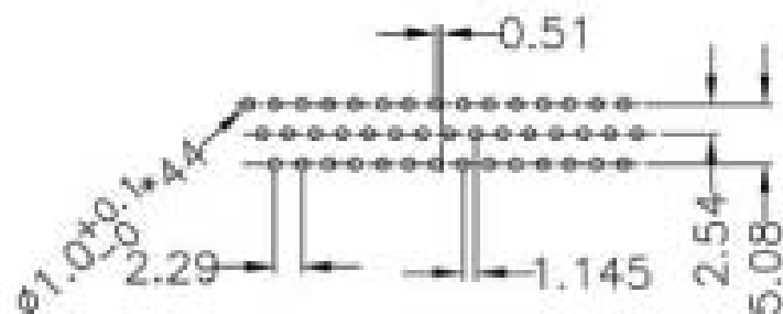
44 Pin Female Connector PCB Pin Layout
