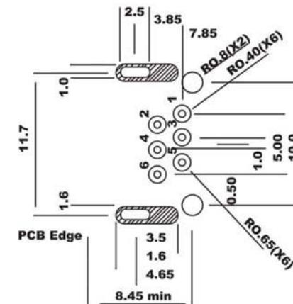
Figure A: PCB Footprint for Receptacle (Through-Hole)
