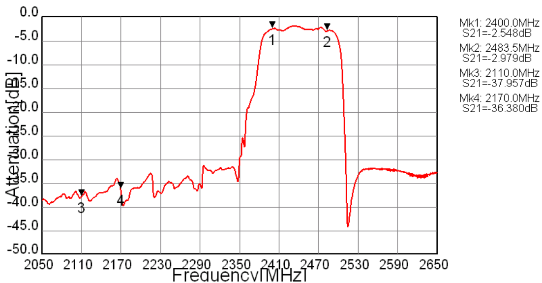
Figure 1. Pass-band Characteristics
