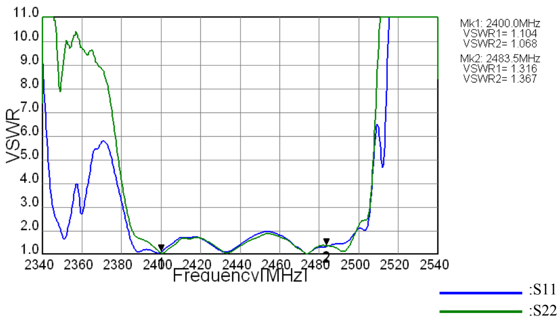
Figure 2. VSWR
