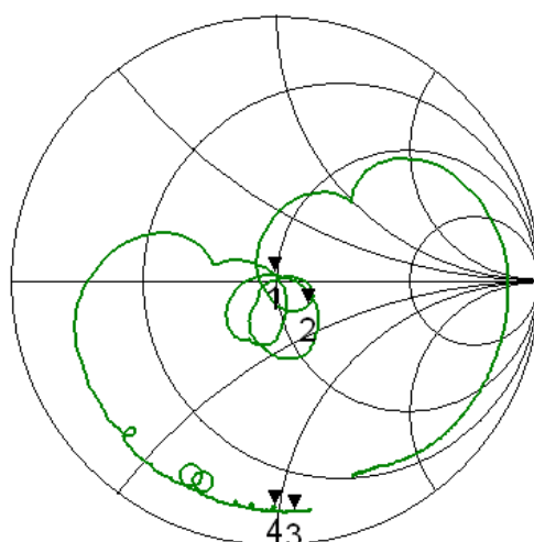
Fig.6 Output Impedance
