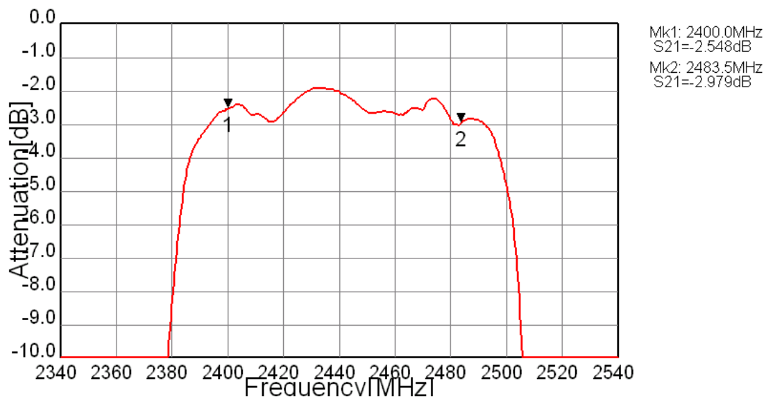
Figure 3. In-band Characteristics
