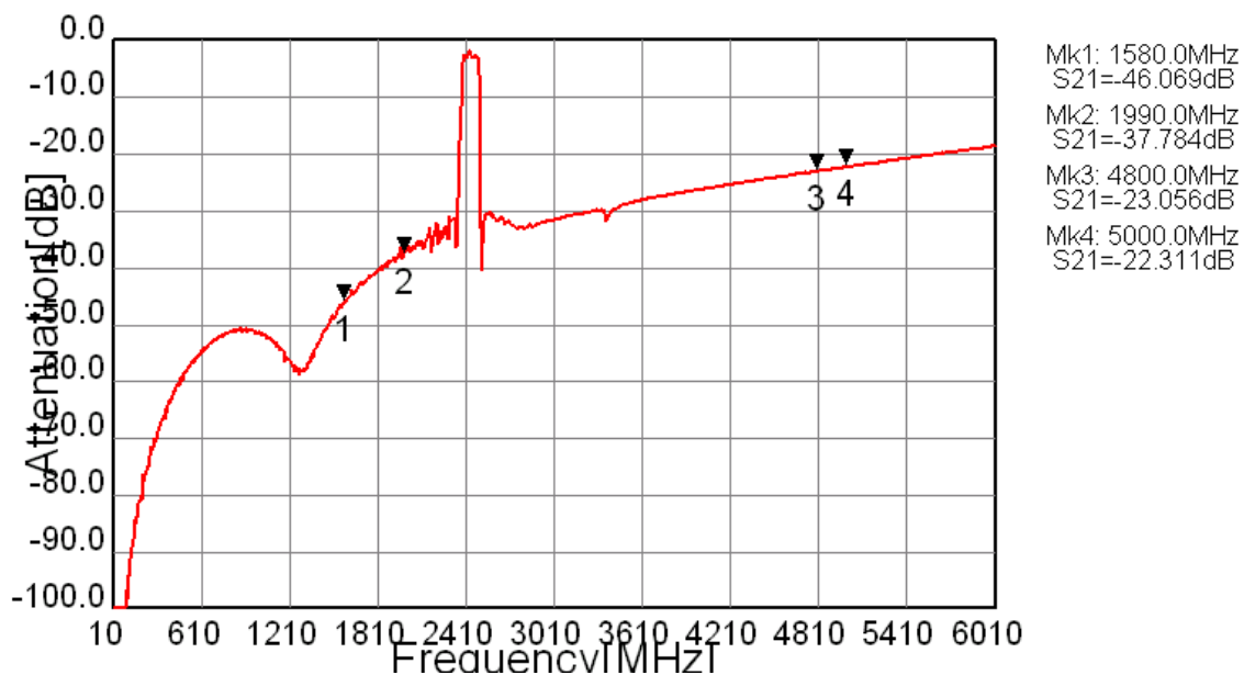
Figure 4. Wide-band Characteristics
