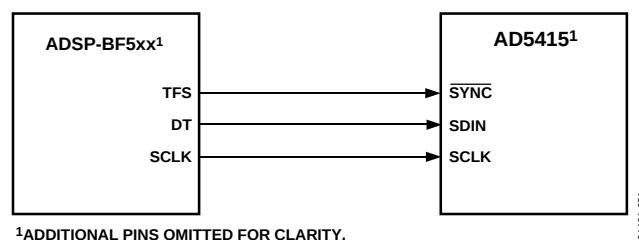
Figure 45. ADSP-BF5xx SPORT-to-AD5415 Interface
