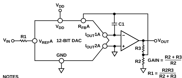
Figure 38. Increasing the Gain of the Current Output DAC
