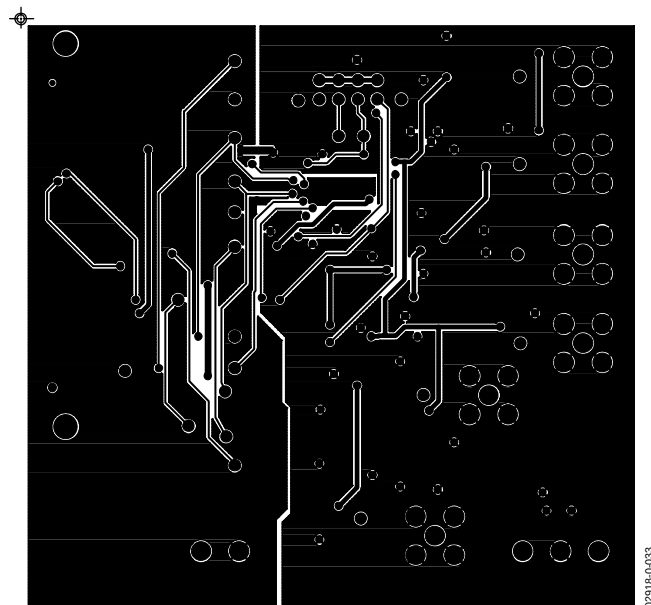
Figure 33. Solder Side
