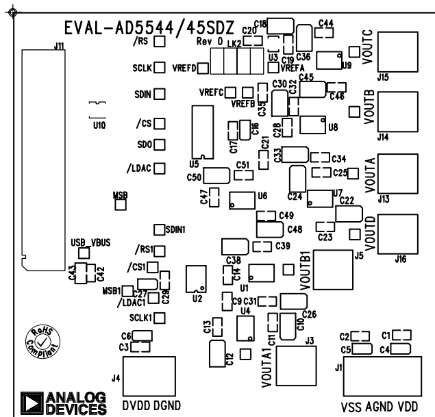
Figure 31. Silkscreen
