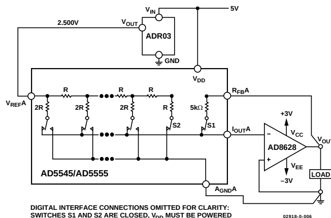
Figure 18. Recommended System Connections
