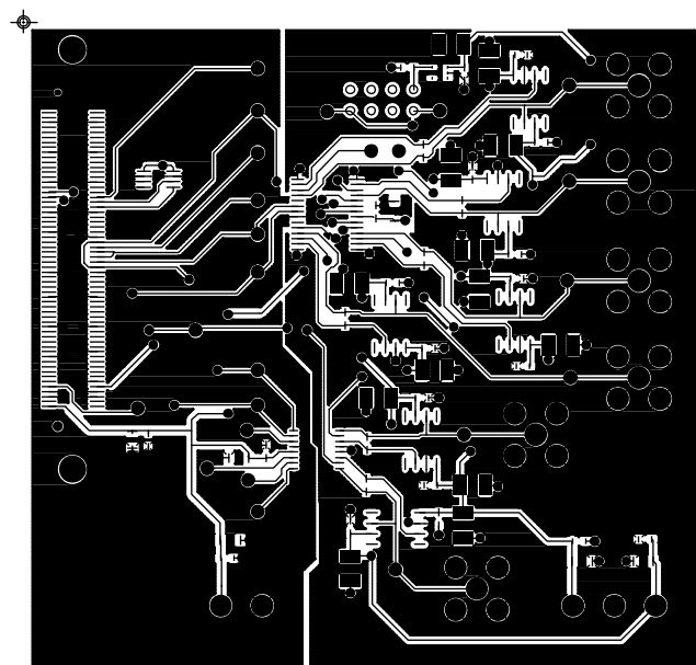
Figure 32. Component Side
