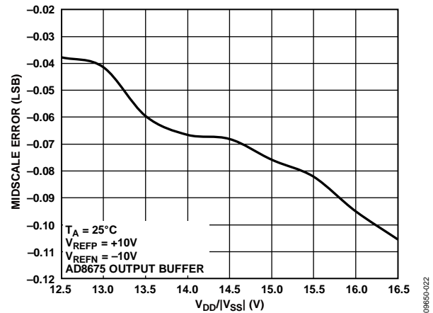
Figure 21. Midscale Error vs. Supply Voltage, \pm 10 V Span
