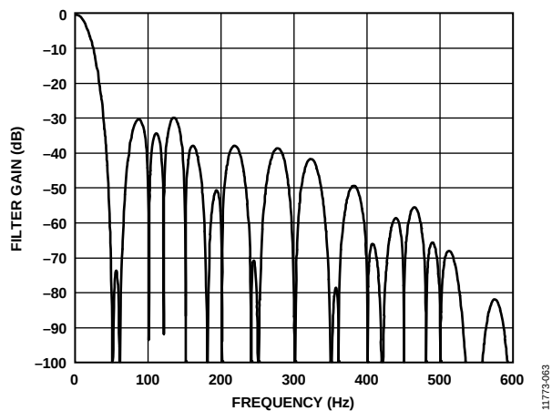
Figure 63. 20 SPS ODR, 50 ms Settling Time
