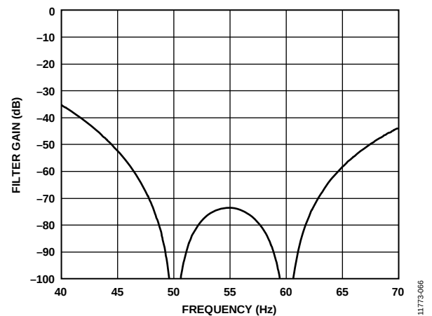
Figure 66. 20 SPS ODR, 50 ms Settling Time
