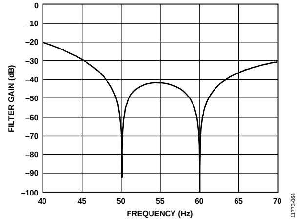
Figure 64. 27.27 SPS ODR, 36.67 ms Settling Time
