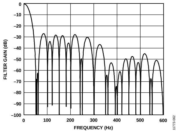
Figure 62. 25 SPS ODR, 40 ms Settling Time
