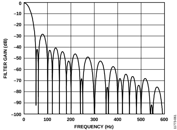
Figure 61. 27.27 SPS ODR, 36.67 ms Settling Time
