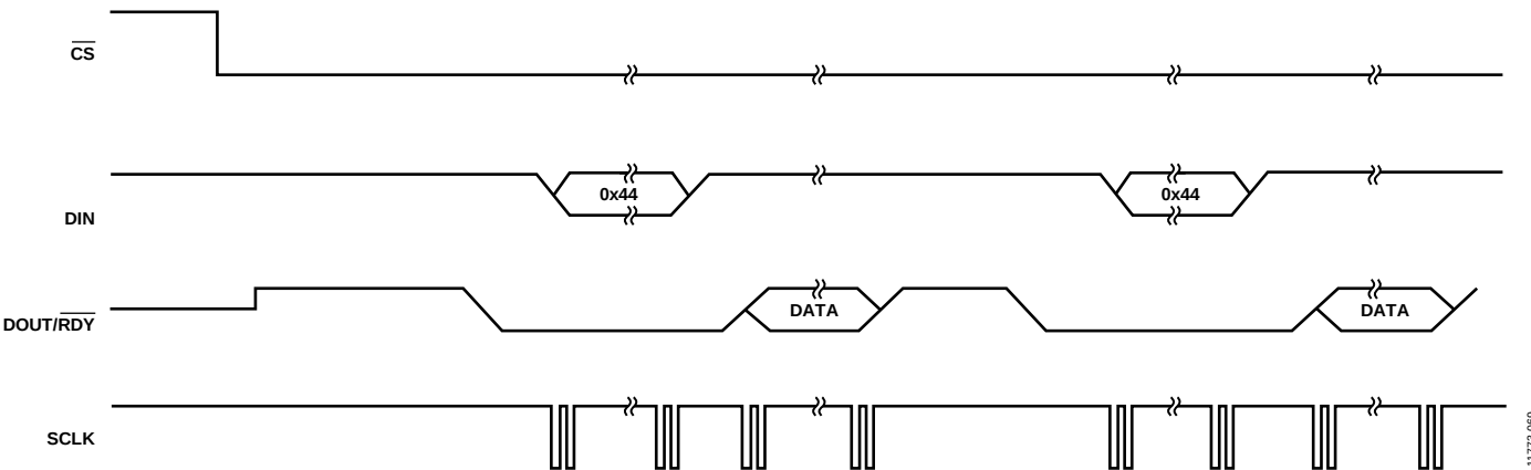
Figure 69. Continuous Conversion Mode
