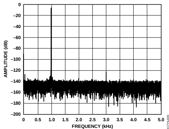
Figure 20. ADC Output FFT; 1 kHz Input Tone, -6 dBFS Input FFT (Output Data Rate = 10 kSPS, External Reference, External Clock, Buffers Enabled)
