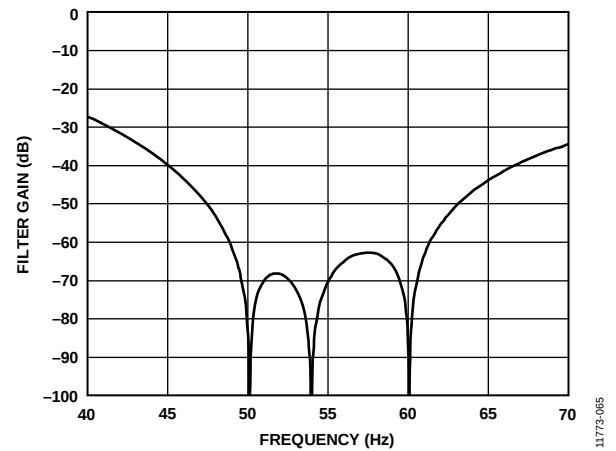
Figure 65. 25 SPS ODR, 40 ms Settling Time
