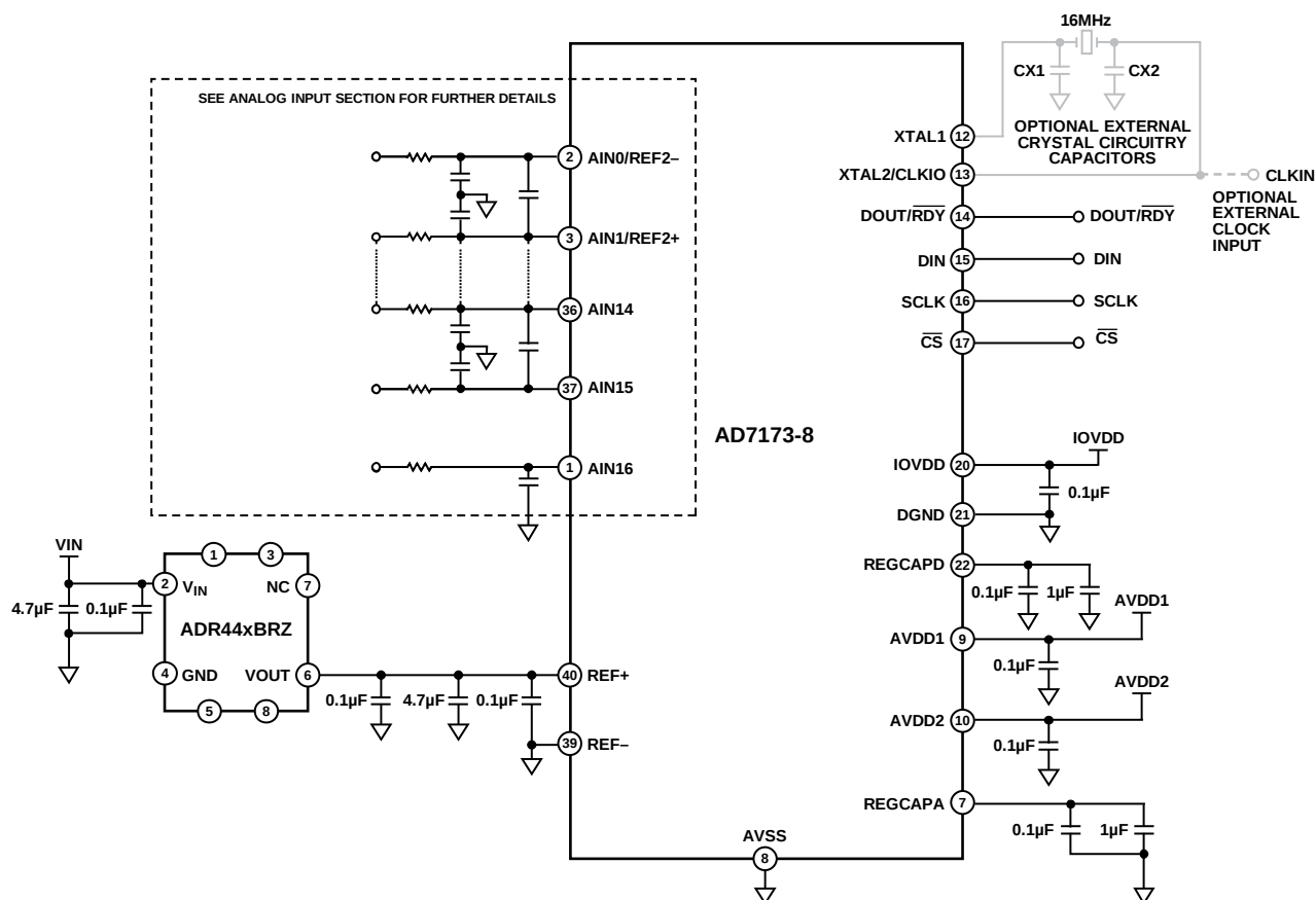
Figure 40. Typical Connection Diagram
