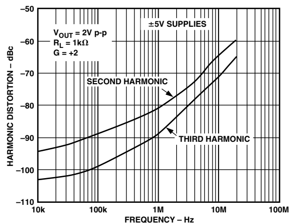
TPC 9. Distortion vs. Frequency, R_L = 1 \text{ k}\Omega
