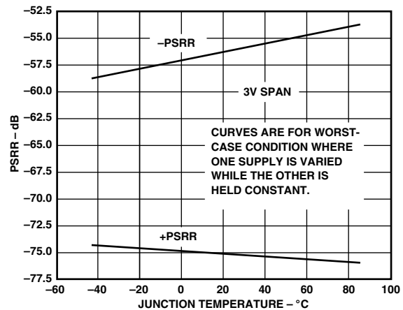
TPC 30. PSRR vs. Temperature
