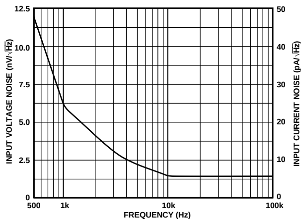
TPC 21. Noise vs. Frequency; V_S = +5\text{ V or } \pm 5\text{ V}
