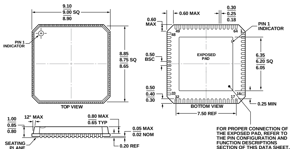
Figure 76. 64-Lead Lead Frame Chip Scale Package [LFCSP_VQ]
