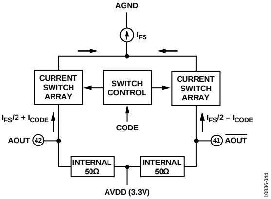
Figure 26. DAC Output
