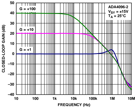
Figure 40. Closed-Loop Gain vs. Frequency
