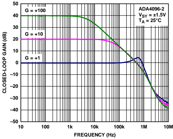
Figure 14. Closed-Loop Gain vs. Frequency
