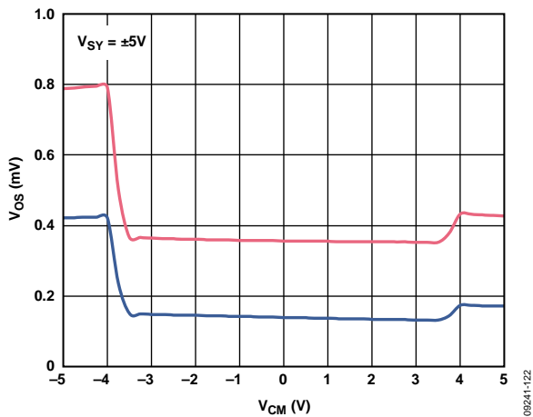
Figure 23. CMRR Sweep, ±10 V
