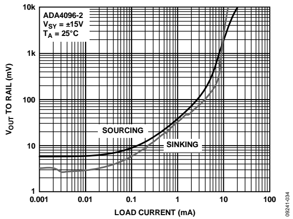
Figure 38. Dropout Voltage vs. Load Current
