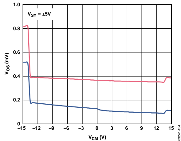
Figure 36. CMRR Sweep, ±30 V
