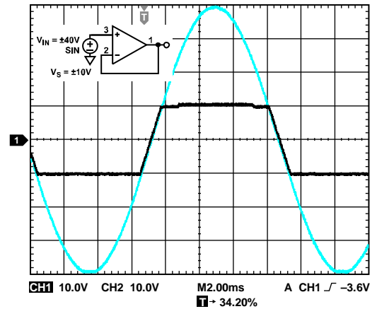
Figure 54. No Phase Reversal
