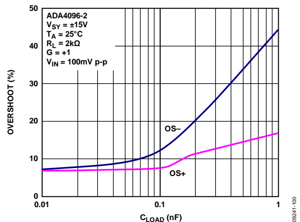
Figure 52. Overshoot vs. Load Capacitance
