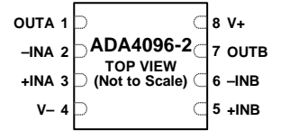
Figure 5. 8-Lead LFCSP (CP-8-10), ADA4096-2
