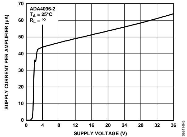
Figure 50. Supply Current vs. Supply Voltage
