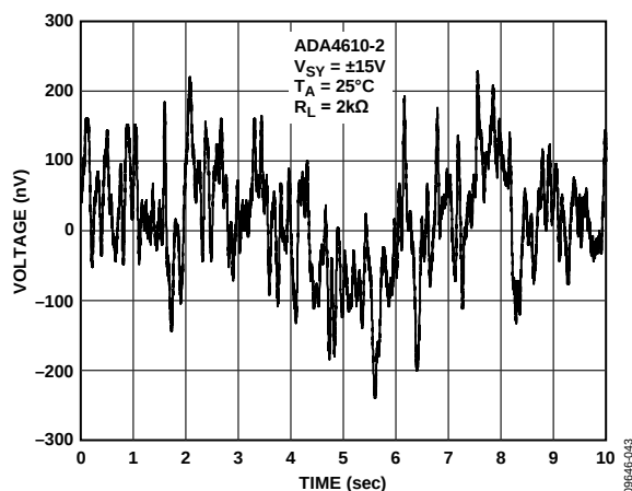
Figure 41. Voltage Noise, 0.1 Hz to 10 Hz
