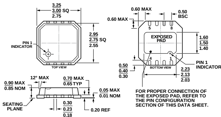
Figure 49. 8-Lead Lead Frame Chip Scale Package [LFCSP_VD]
