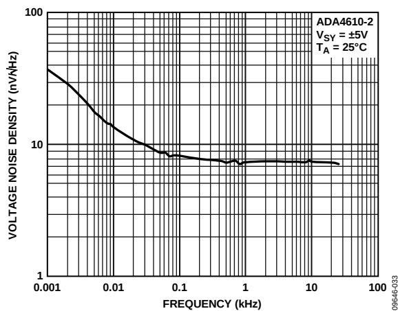
Figure 32. Voltage Noise Density
