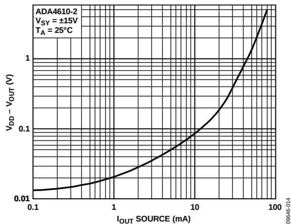
Figure 17. Dropout Voltage vs. Source Current
