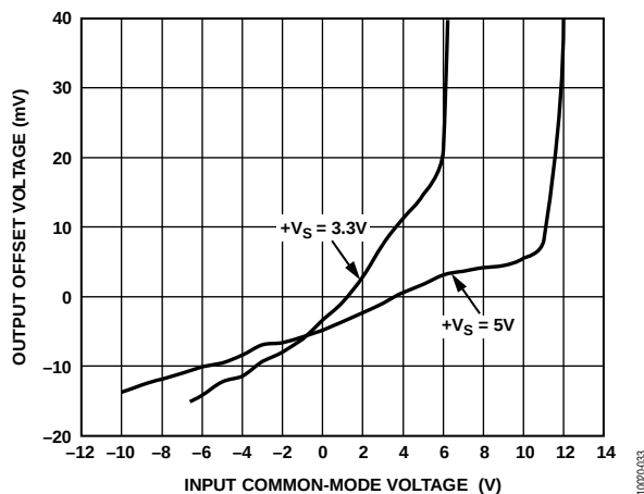
Figure 21. Output Offset Voltage ( V_{OUT} - V_{REF} ) vs. Input Common-Mode Voltage
