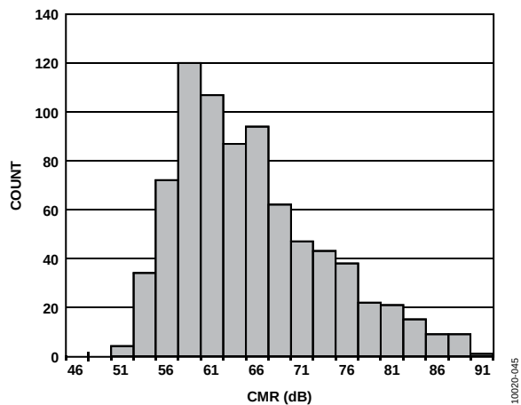
Figure 23. Typical Distribution of Common-Mode Rejection
