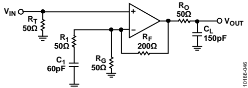
Figure 43. Configuring the ADA4895-2 for a Gain of +5 Stable
