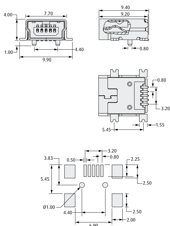
Recommended PC Board Pattern
