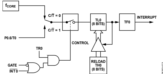
Figure 84. Timer/Counter 0, Mode 2
