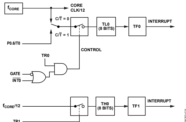
Figure 85. Timer/Counter 0, Mode 3
