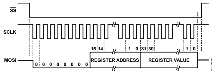
Figure 90. SPI Write Operation of a 32-Bit Register
