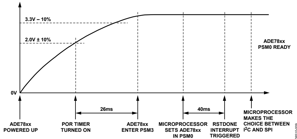
Figure 26. Power-Up Procedure
