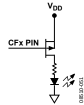
Figure 76. CFx Pin Recommended Connection
