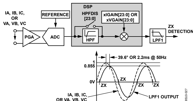
Figure 43. Zero-Crossing Detection on Voltage and Current Channels
