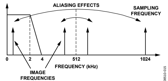
Figure 32. Aliasing Effects
