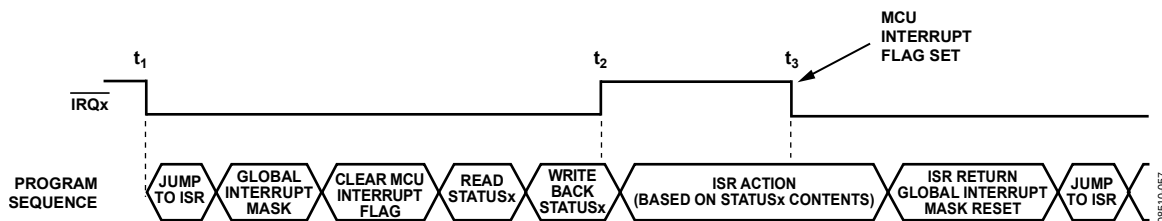
Figure 84. Interrupt Management
