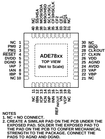
Figure 9. Pin Configuration
