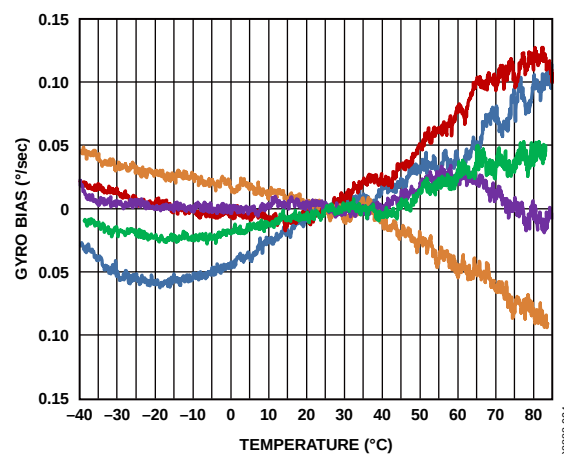
Figure 9. Bias vs. Temperature, 0.1°C/Min Ramp Rate, Autonull at +25°C, SMPL_PRD = 0x001F, DEC_RATE = 0x0010
